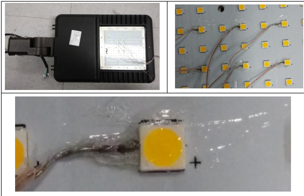
Thermocouple Location on Temperature Measurement Point (TMP):
