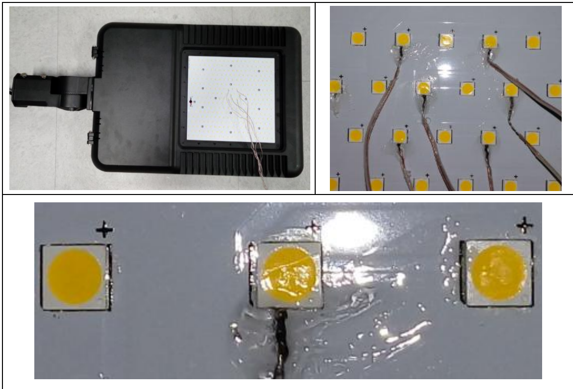
Thermocouple Location on Temperature Measurement Point (TMP):
