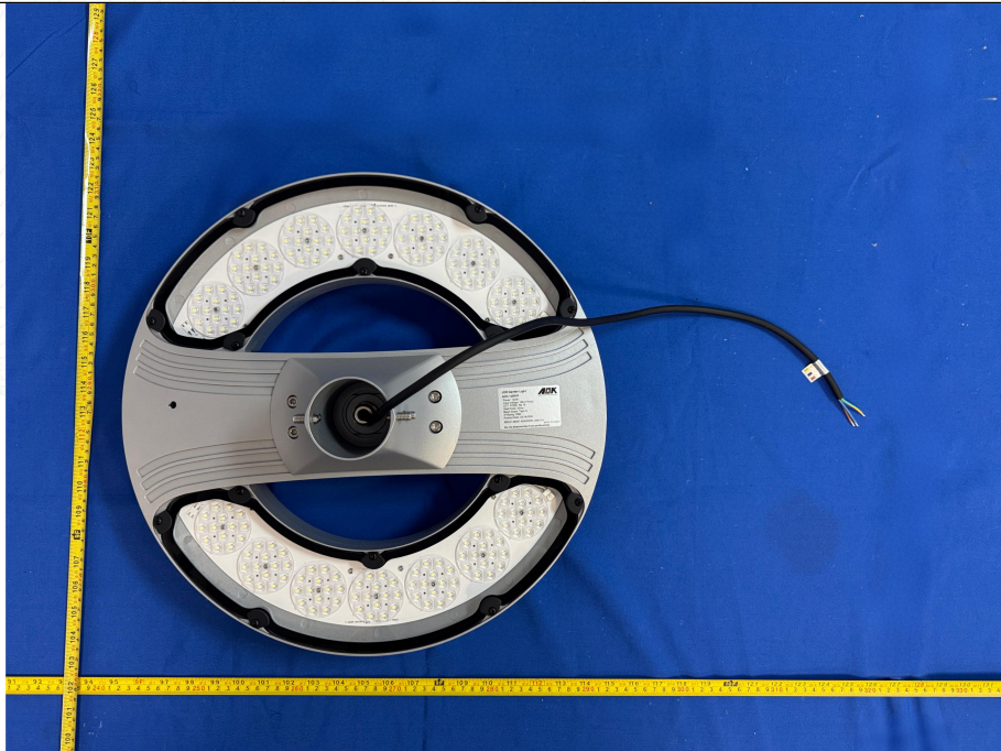
Photo 1: Overall view of model AOK-120WIP-NV-L2-00-6570-T4-P
