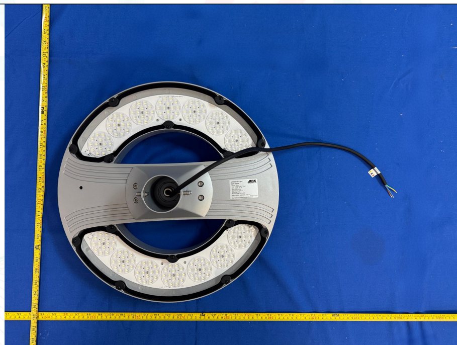
Photo 2: Overall view of model AOK-120WIP-NV-L2-00-6570-T4-P
