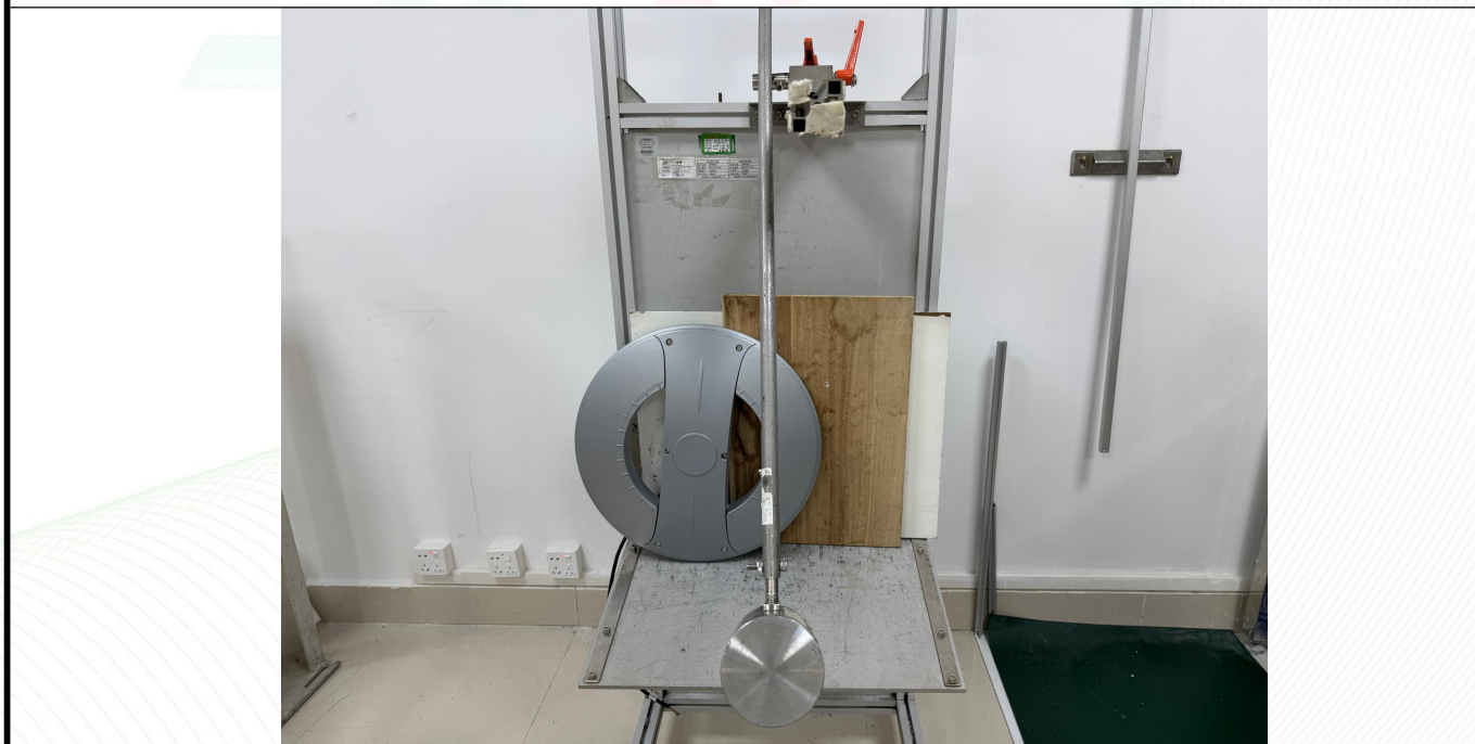
Photo 4: IK09 test of model AOK-120WIP-NV-L2-00-6570-T4-P
